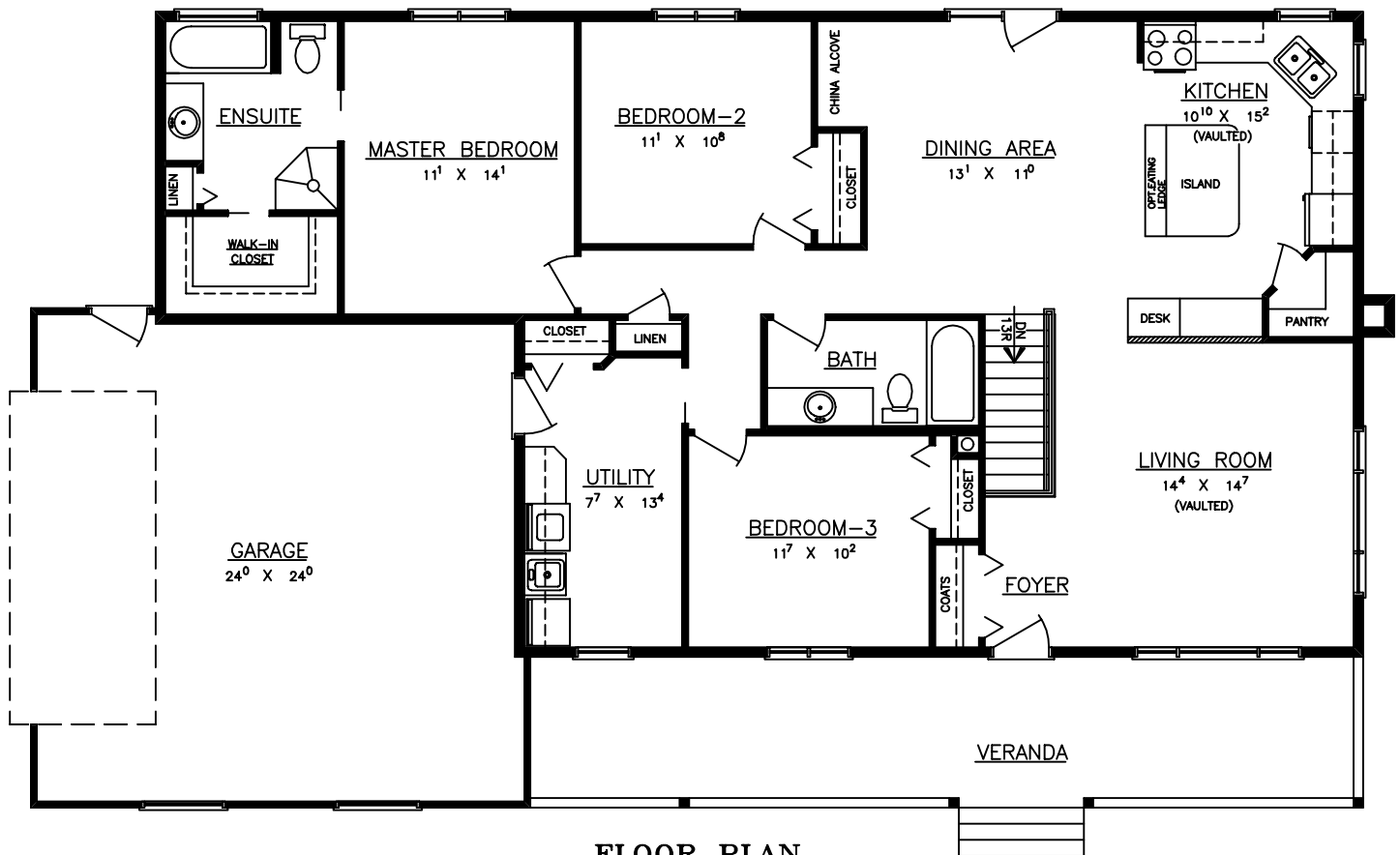
FLOOR PLAN
